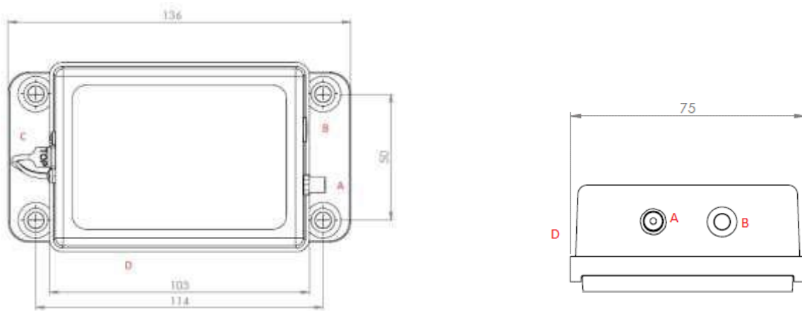
Example - GPS unit without mounting points
